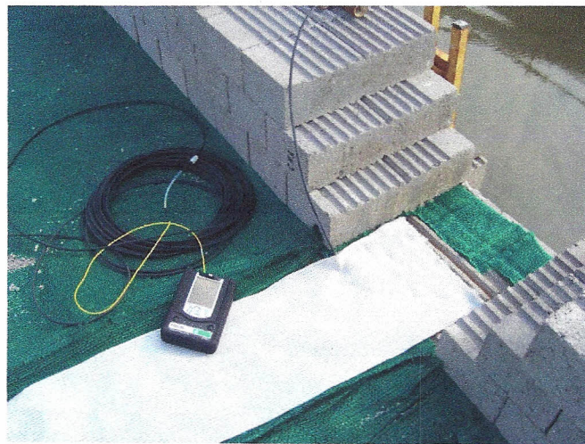
Figure 3: The GeoDetect® strip No. 2 installed.
