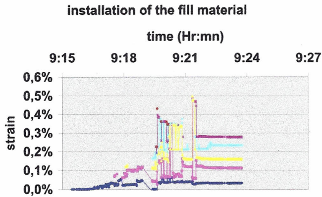
Figure 4: Measurement during installation of strip No. 1.
