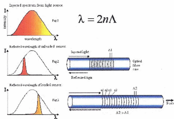
Figure 1: FBG response as function of strain.
