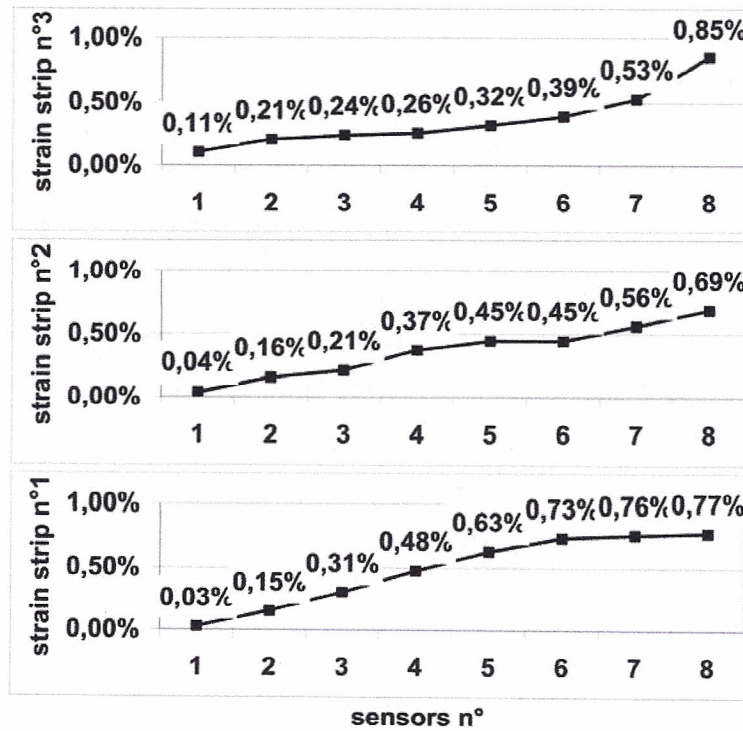
Figure 7: Strain profiles of the 3 strips – June 2005.
