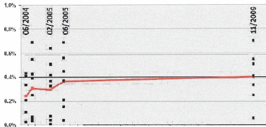
Figure 8: Sensor readings from initial construction in 2004 to several years after completion in 2009.
