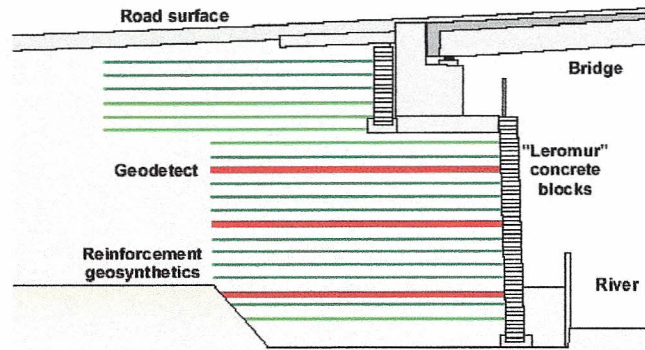
Figure 2: Distribution of strips within the northern abutment.
