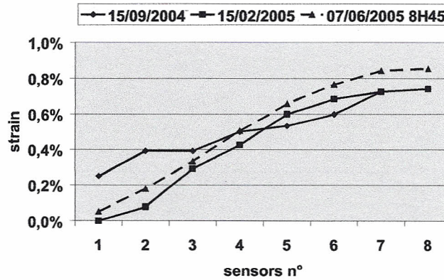
Figure 6: Strain profiles of strip No. 1 at different times.
