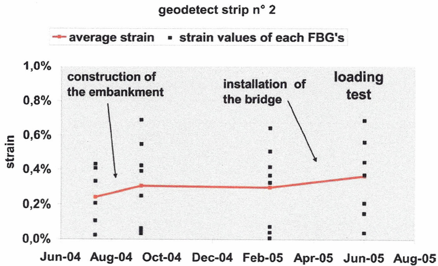
Figure 5: Evolution of strains measured on strip No. 2.
